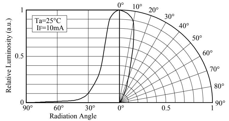
■ Directivity (NSPE510(S))
